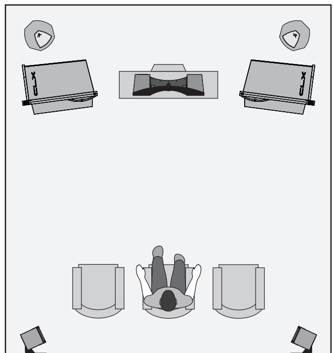
Figure 13. CLX speakers as front channels, the Stage as the center and surround channels, and Descent i subwoofers as 0.1 (effects) channel.
